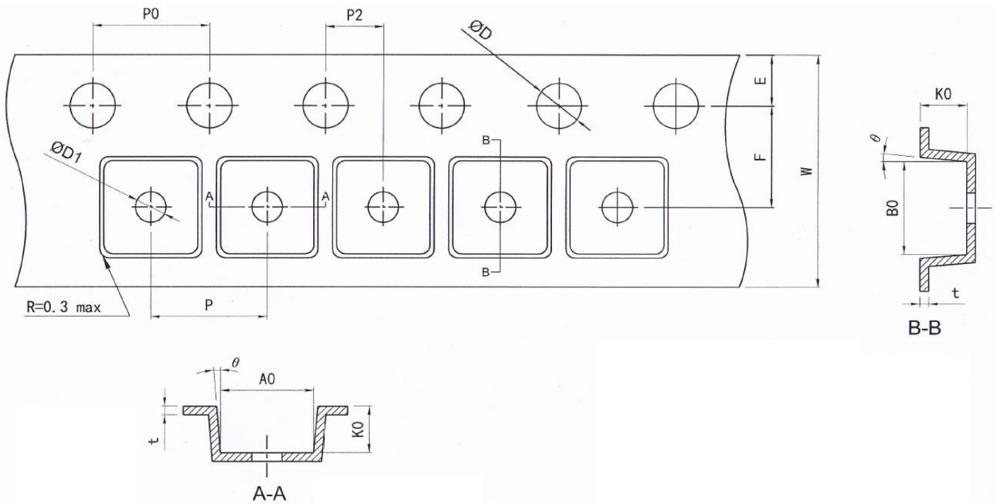
Dimensions In Millimeters
