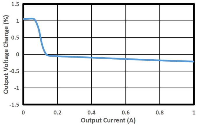
Figure 4. Load Regulation ( V OUT =12V, L=47μH)
