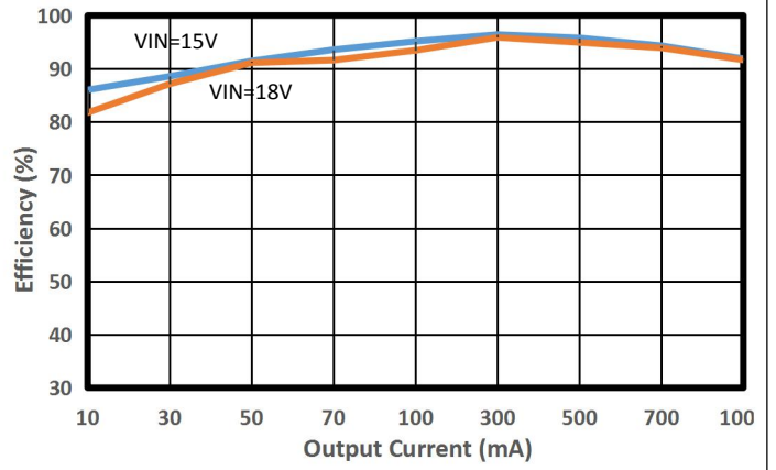
Figure 2. Efficiency vs. Load Current ( V OUT =12V, L=47μH)
