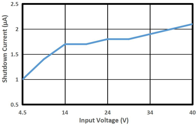
Figure 3. Input Voltage vs. Shutdown Current ( V OUT =5V)
