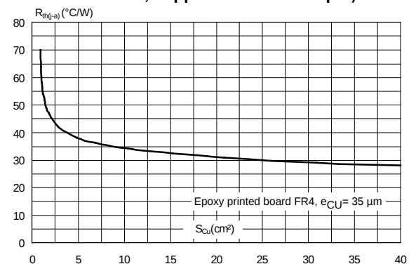
Figure 12: Thermal resistance junction to ambient versus copper surface under tab (printed circuit board FR4, copper thickness: 35 \mu m )
