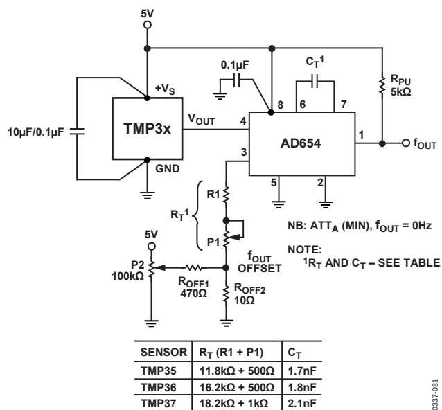
Figure 34. Temperature-to-Frequency Converter
