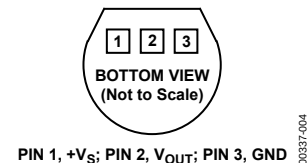
Figure 4. T-3 (TO-92)
