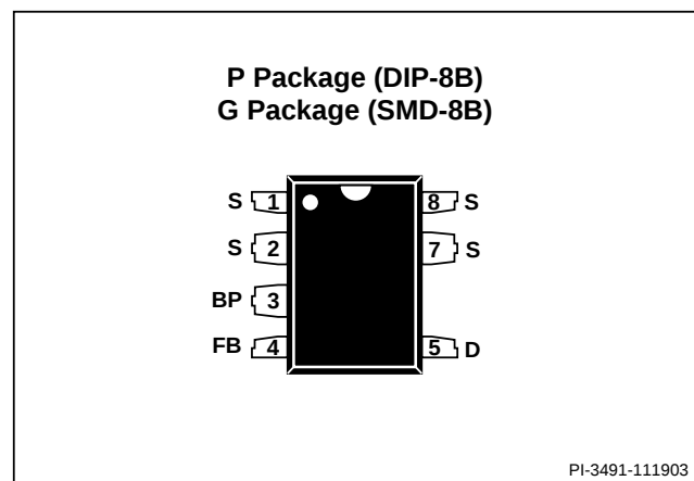
Figure 3. Pin Configuration.
