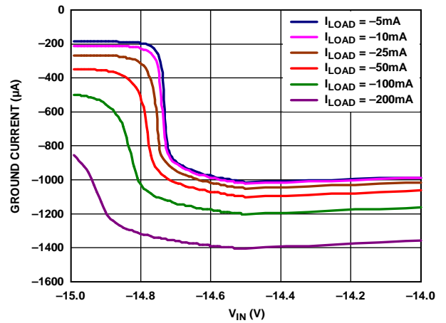
Figure 48. Ground Current vs. Input Voltage ( V_{IN} ) in Dropout, V_{OUT} = -15\text{ V}
