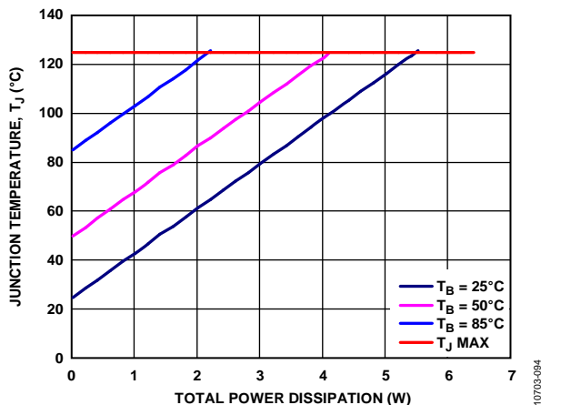
Figure 100. Junction Temperature vs. Total Power Dissipation for the 5-Lead TSOT, T_A = 85^\circ\text{C}
