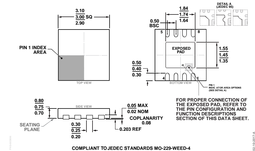
Figure 105. 8-Lead Lead Frame Chip Scale Package [LFCSP] 3 mm × 3 mm Body and 0.75 Package Height (CP-8-13) Dimensions shown in millimeters
