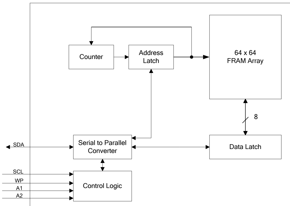
Figure 1. Block Diagram
