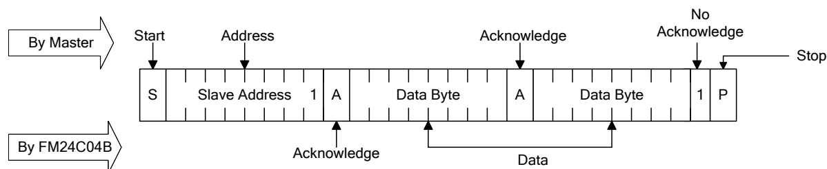
Figure 8. Sequential Read
