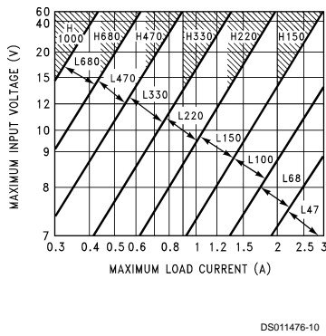
FIGURE 4. LM2576(HV)-5.0
