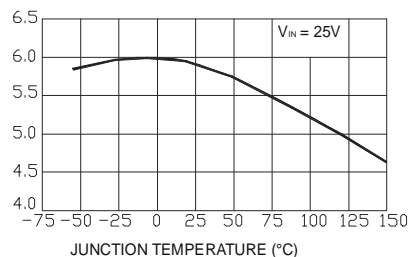
Oscillator Frequency
