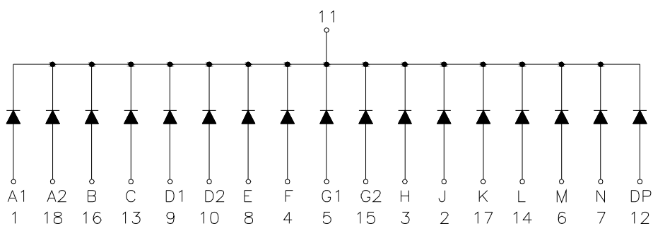
Common Cathode
