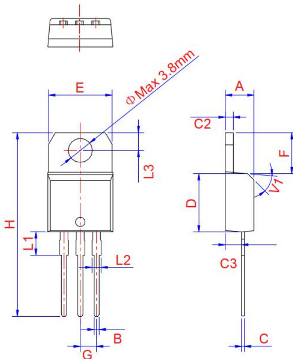
TO-220B Non-Ins
