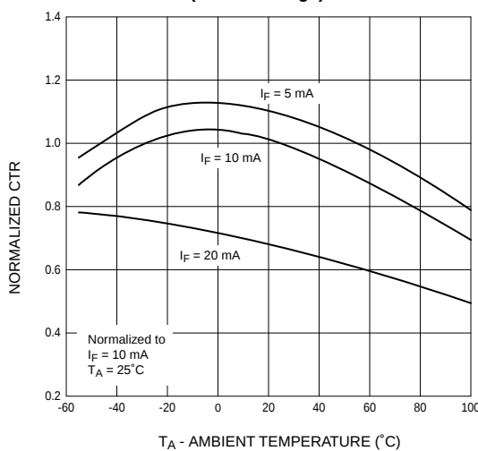
Fig. 4 Normalized CTR vs. Ambient Temperature (White Package)
