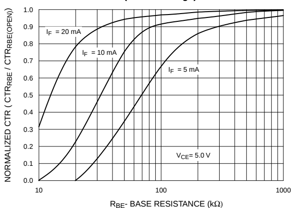
Fig. 6 CTR vs. RBE (Unsaturated) (White Package)
