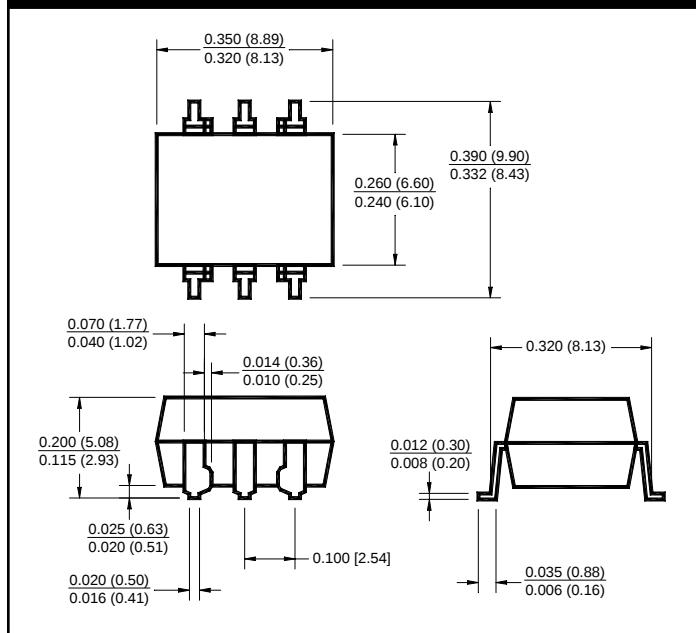
Package Dimensions (Surface Mount)
