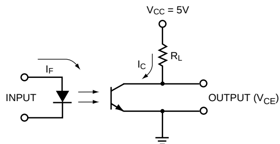
Figure 19. Switching Time Test Circuit
