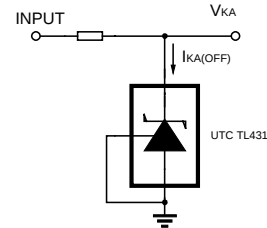
For I_{KA(OFF)}
