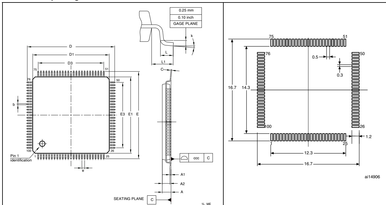
Figure 42. Recommended footprint (1)(2)
