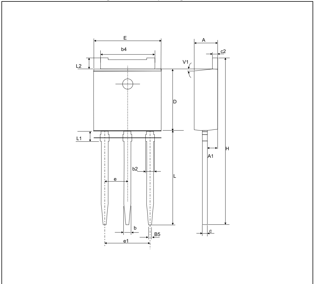
Figure 13. IPAK package outline
