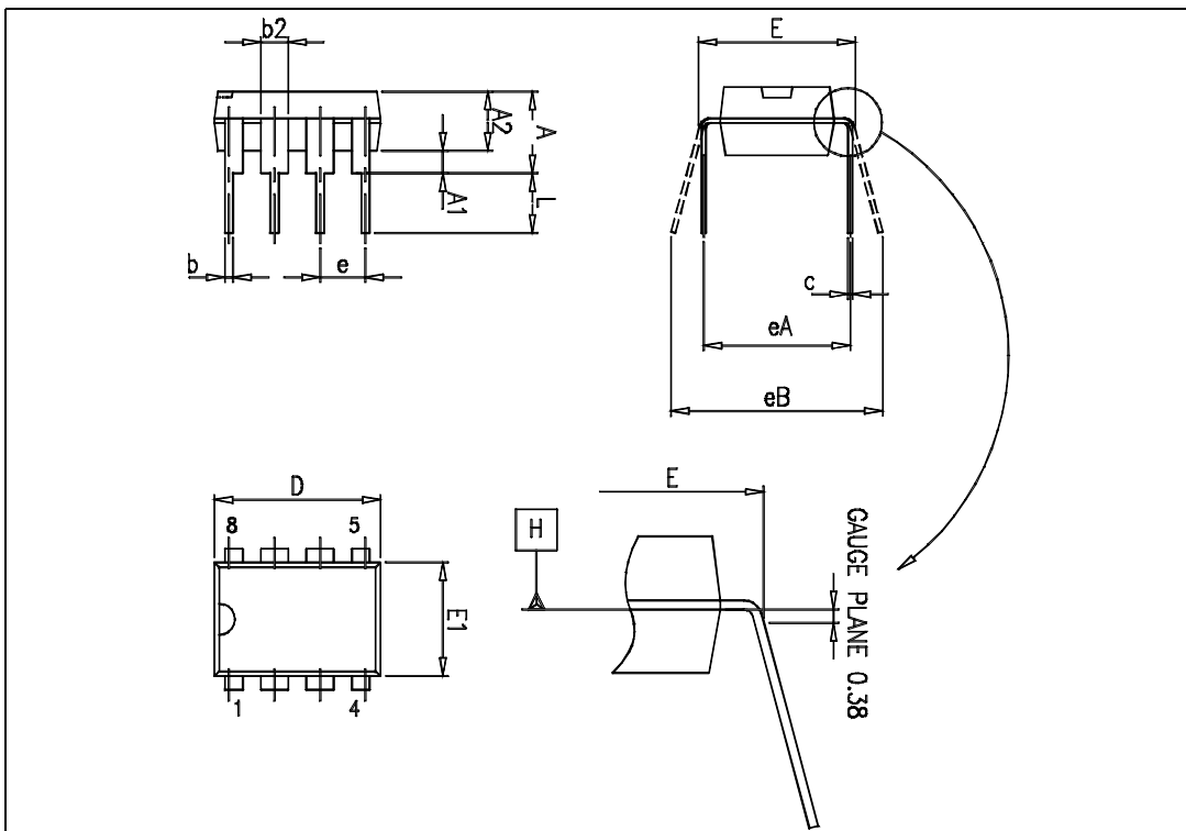
Figure 15. Package Dimensions
