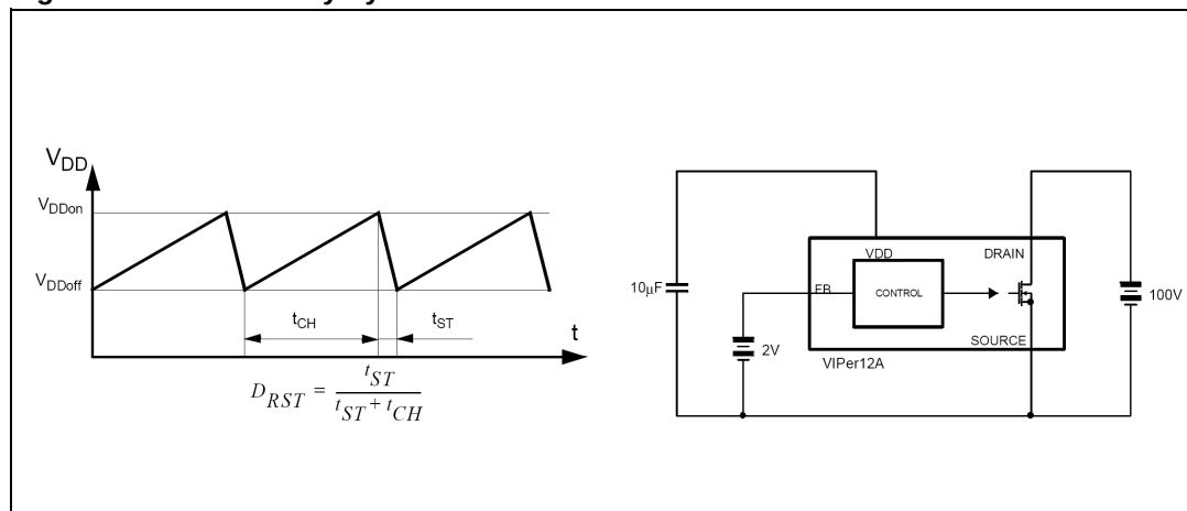
Figure 10. Restart duty-cycle
