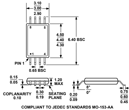
COMPLIANT TO JEDEC STANDARDS MO-153-AA Figure 71. 8-Lead Thin Shrink Small Outline Package [TSSOP] (RU-8) Dimensions shown in millimeters
