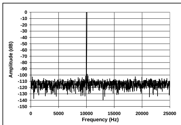
FIGURE 2-19: Frequency Spectrum of 10 kHz Input (Representative Part).
