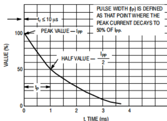
Figure 5. Pulse Waveform
