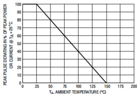
Figure 6. Pulse Derating Curve
