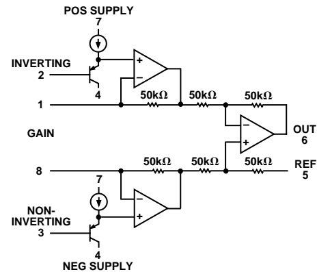
Figure 40. Simplified Schematic
