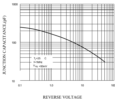
FIG.5-TYPICAL JUNCTION CAPACITANCE
