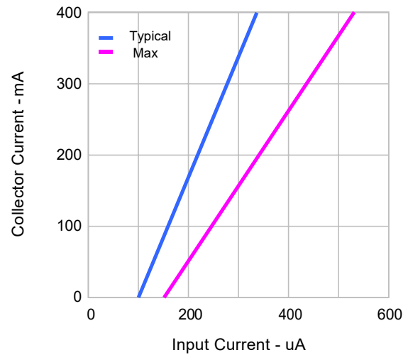
Figure 2. Collector Current vs. Input Current
