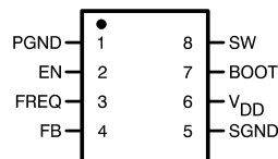
Figure 2. Top View
