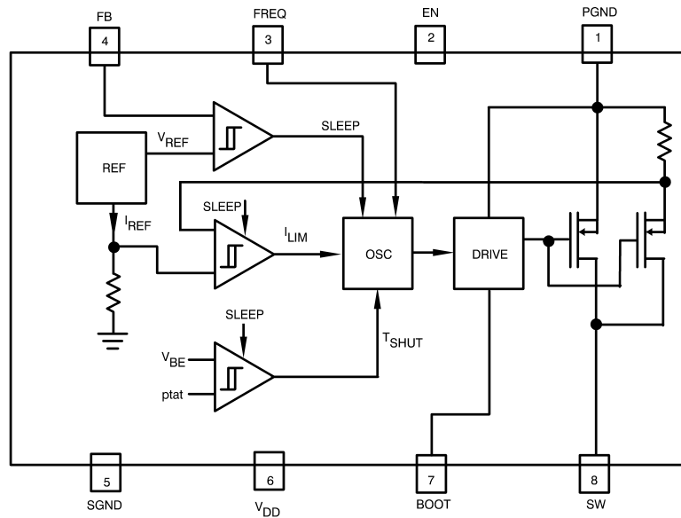
Figure 3. Functional Diagram
