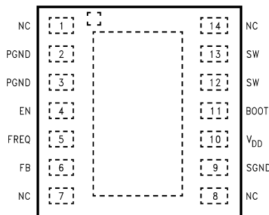
Figure 1. Top View
