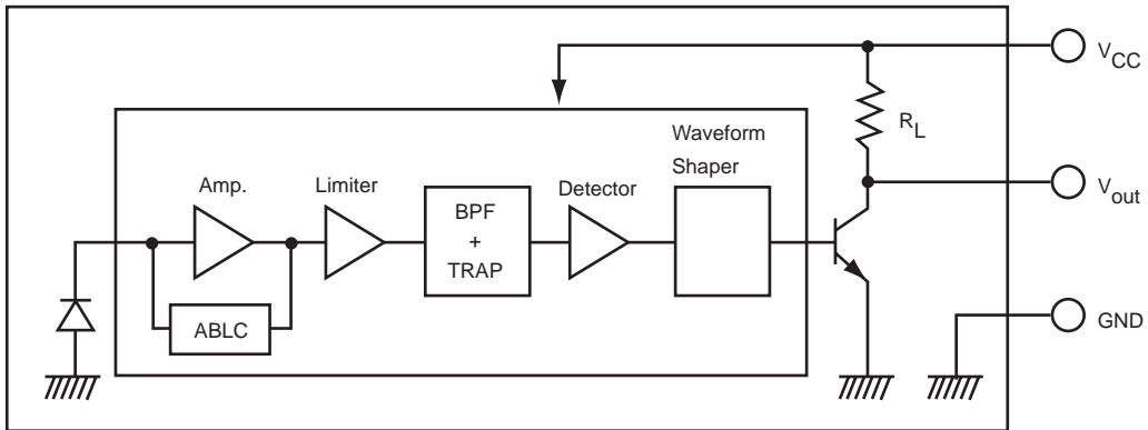
Fig.4 Block Diagram
