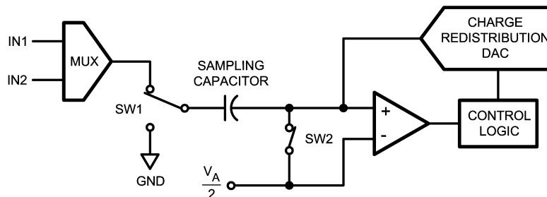
FIGURE 1. ADC122S101 in Track Mode
