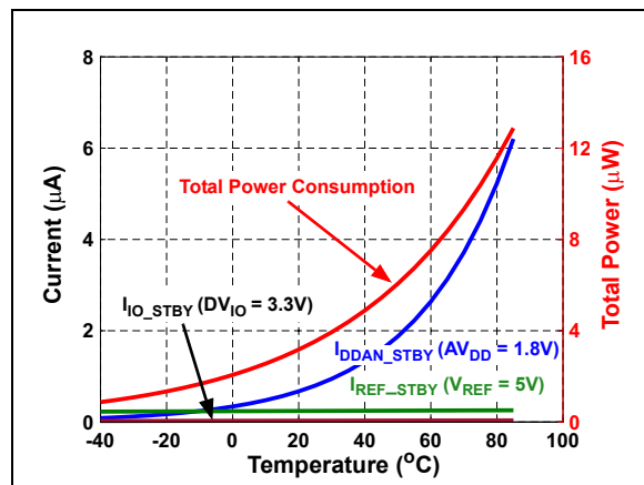
FIGURE 4-35: Power Consumption vs. Temperature during Shutdown.
