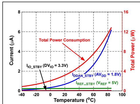
FIGURE 3-35: Power Consumption vs. Temperature during Shutdown.
