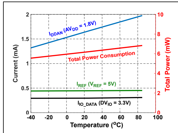
FIGURE 3-34: Power Consumption vs. Temperature: C_{LOAD\_SDO} = 20\text{ pF} .
