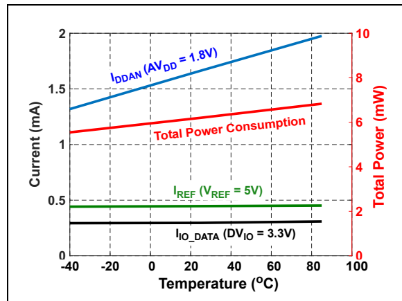
FIGURE 4-34: Power Consumption vs. Temperature: C_{LOAD\_SDO} = 20\text{ pF} .
