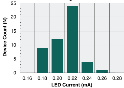
Typical I_F for Switch Operation (N=50, I_L=600mA )
