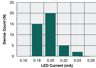
Typical I_F for Switch Dropout (N=50, I_L=600mA )
