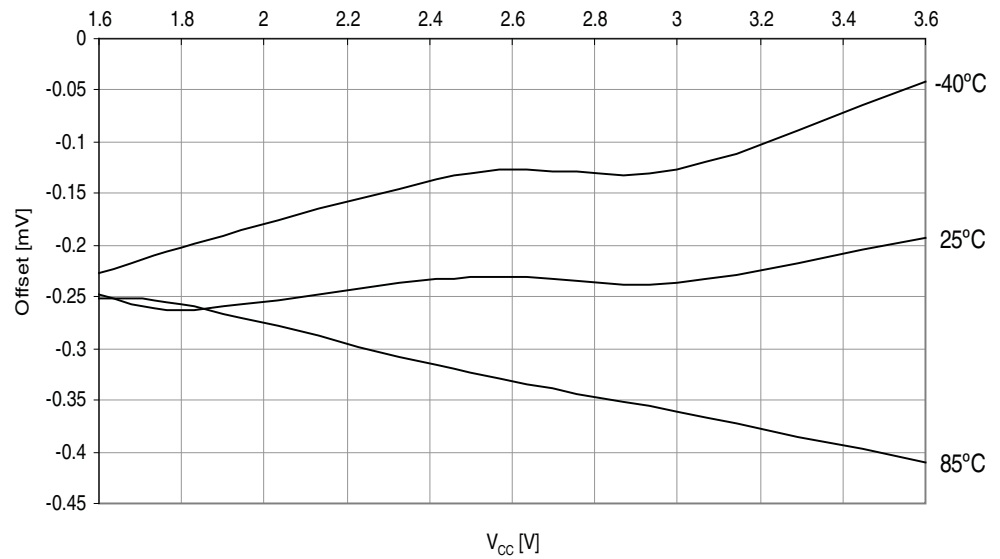
Figure 36-46. Offset vs. V_{CC}
