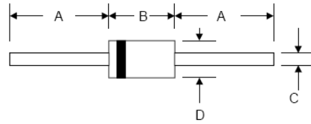
DO-15
