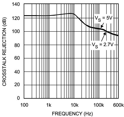
Crosstalk Rejection vs. Frequency (LMV772/LMV774)
