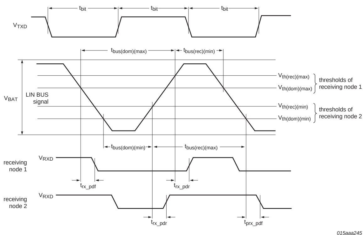
Fig 6. Timing diagram LIN transceiver
