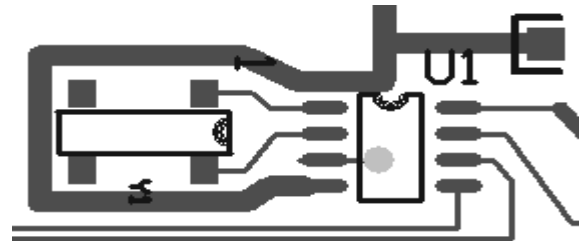
FIGURE 19. SUGGESTED LAYOUT FOR ISL1208 AND CRYSTAL
