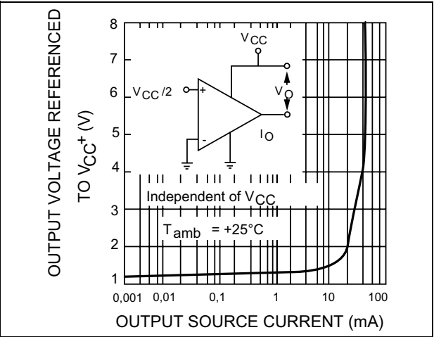
Figure 7. Output characteristics
