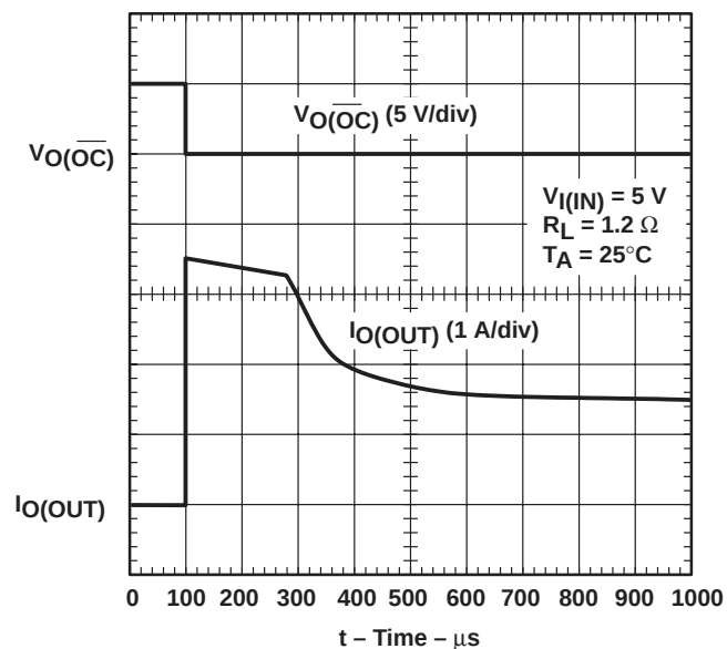
Figure 18. 1.2\text{-}\Omega Load Connected to an Enabled TPS2022 Device
