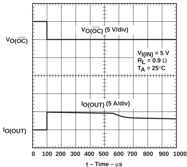
Figure 21. 0.9\text{-}\Omega Load Connected to an Enabled TPS2024 Device
