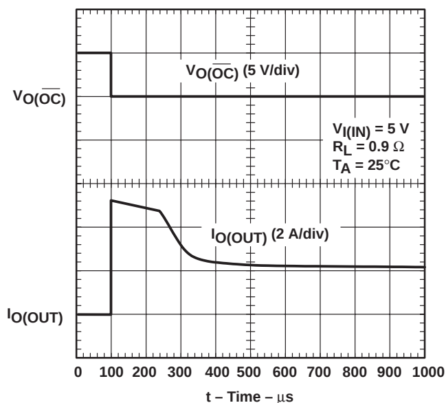
Figure 20. 0.9\text{-}\Omega Load Connected to an Enabled TPS2023 Device
