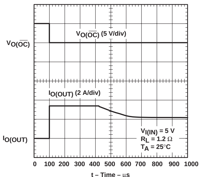
Figure 19. 1.2\text{-}\Omega Load Connected to an Enabled TPS2023 Device
